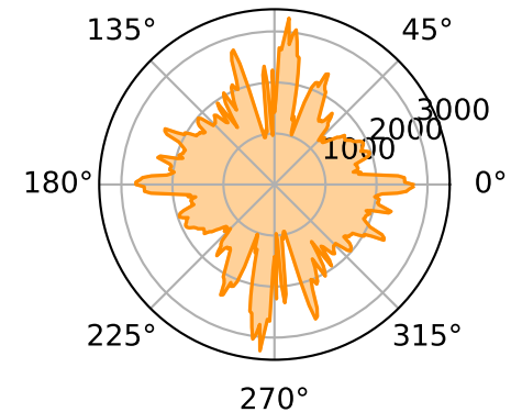
Chirality per angular sector
