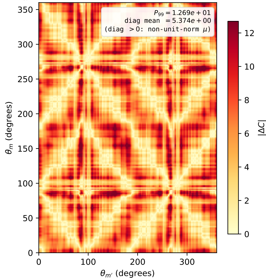
D_\chi : |C(m, m') - C(-m, -m')| (saturated at P_{99} )
