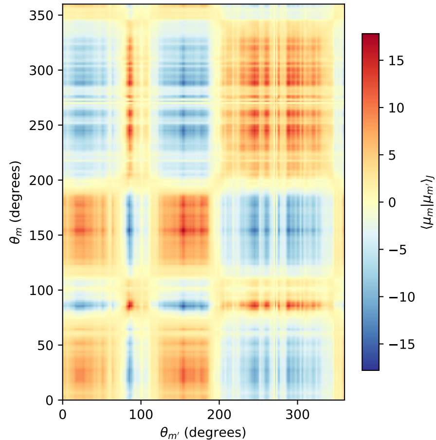
C_\mu : Jacobian Correlation of Micro-space
